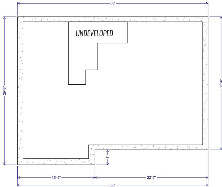
BASEMENT
