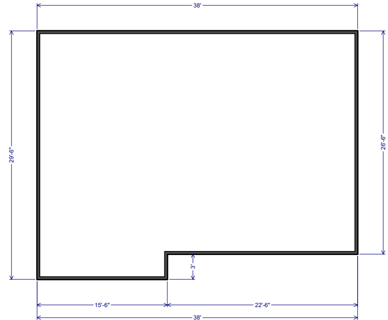
MAIN LEVEL
